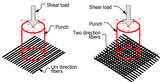
Figure 8. Sketch shear load on the fiber direction
